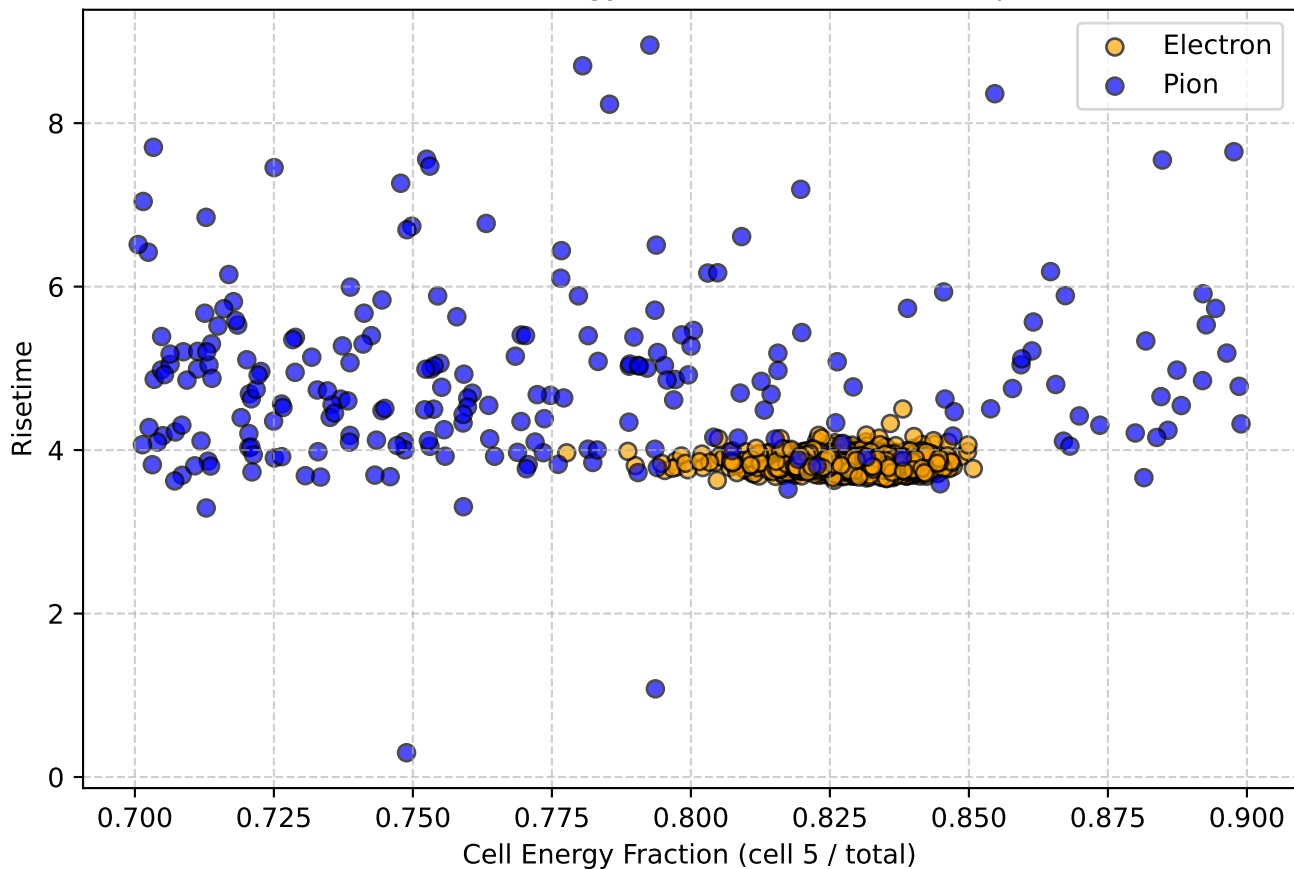
Risetime vs Cell Energy Fraction for 100.0GeV particles
